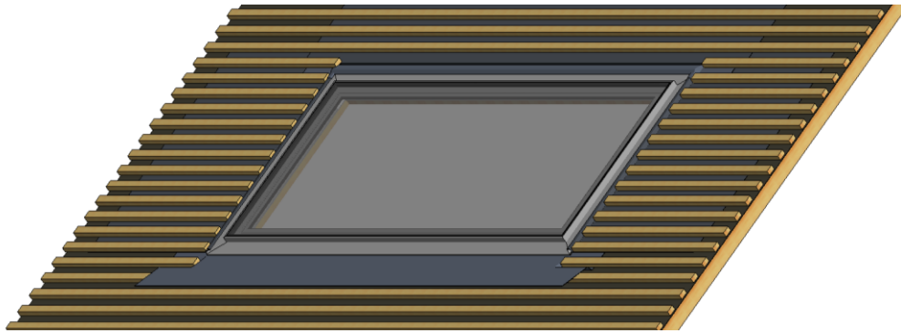
Figure 11 – Battens installed
