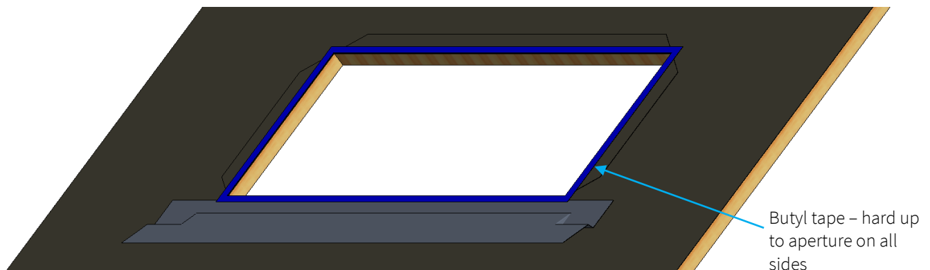
Figure 4b – Continuous loop of butyl tape applied on top of underlay
